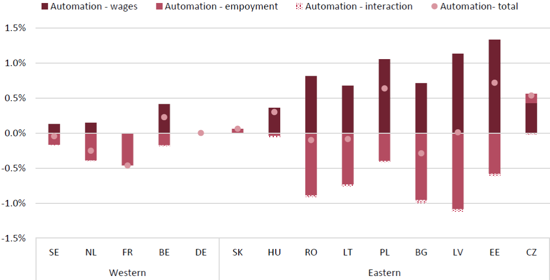
Figure 10. The difference between country-specific and German automation-driven changes in the Gini Index
