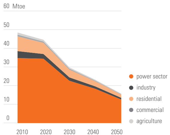
Figure 22. Coal consumption by sector
