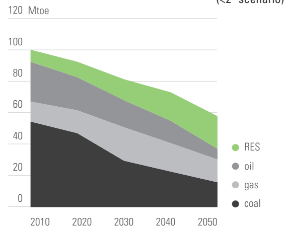
Figure 20. Total Primary Energy Supply by source (<2° scenario)
