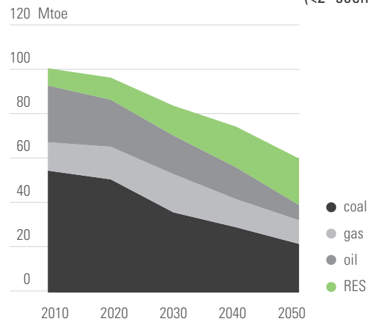
Figure 17. Total Primary Energy Supply the source
